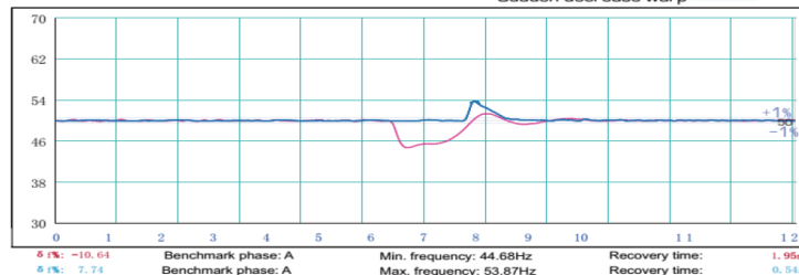
Sudden frequency warp
