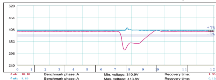
Sudden voltage warp
